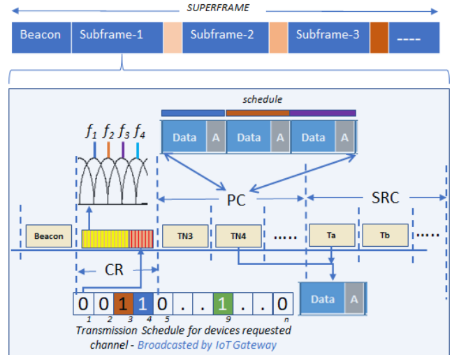
Fig. 2. Superframe structure
