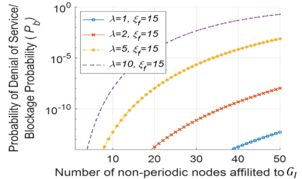
Fig. 6. P_b as a function of affiliated non-periodic nodes
