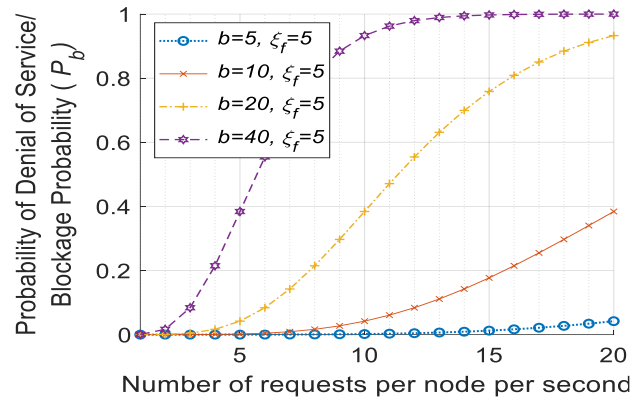
Fig. 5. P_b with changing requests per node per second ( \lambda )
