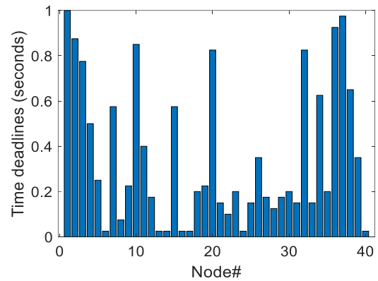
Fig. 3. Periodic communication interval of different sensor nodes
