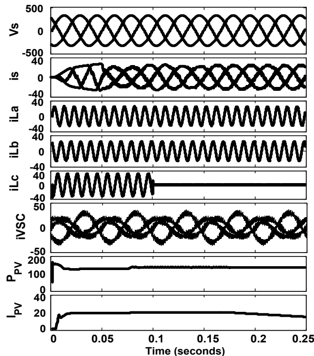
Fig. 14. System behavior showing source, load, and filter current with PV power and current, under unbalanced non-linear load using ANF-RLS.
