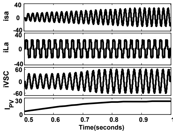
Fig. 20. Dynamic response of the system for increase in solar insolation.
