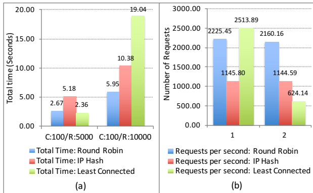
Fig. 10. Benchmarking: Comparison between round robin, IP hash and least connected load balancing algorithms
