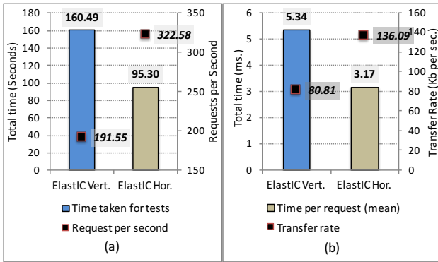
Fig. 12. Comparison between vertical and horizontal autoscaling performance during run-time execution of 30,000 HTTP requests
