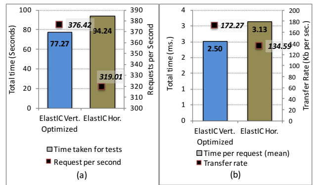
Fig. 13. Comparison between optimized vertical and horizontal autoscaling performance during run-time execution of 30,000 HTTP requests
