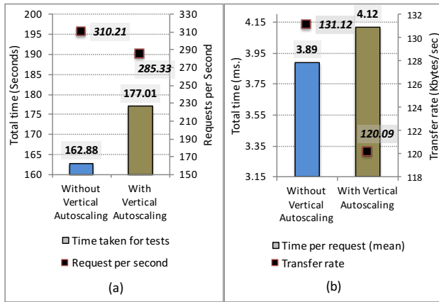
Fig. 18. Comparison between total time of tests, requests per second, time per request and transfer rate for the two cases of vertical and non-vertical autoscaling
