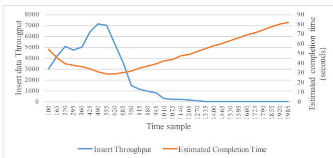
Fig. 2. YCSB Elasticsearch workload insert throughput data failure and estimation completion time for small size VM (10 million tasks for insert and update records)
