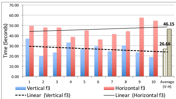
Fig. 7. Horizontal versus vertical autoscaling of a cloud App for flavor f3
