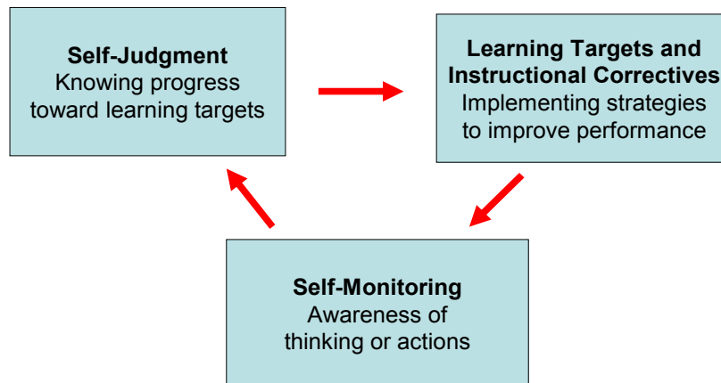
Figure 2. Self-assessment Cycle
